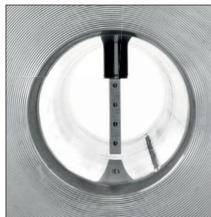
Averaging pitot tube
